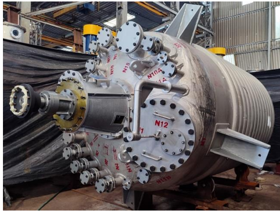
REACTOR
